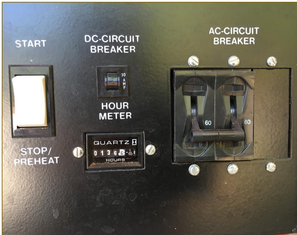
Figure 53 - Kohler Generator Control Panel, 136 hours.
