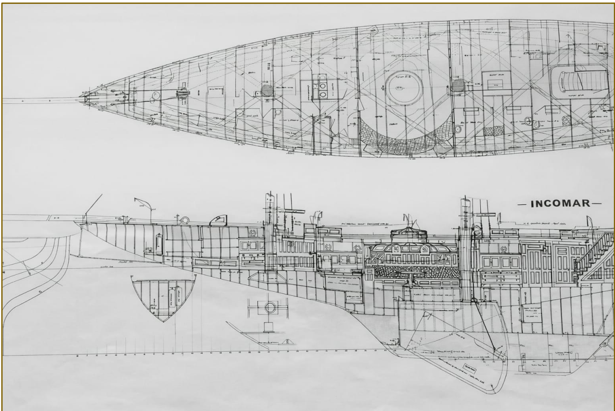
Figure 3 – Part of the original N.G. Herreshoff plans for Ingomar
