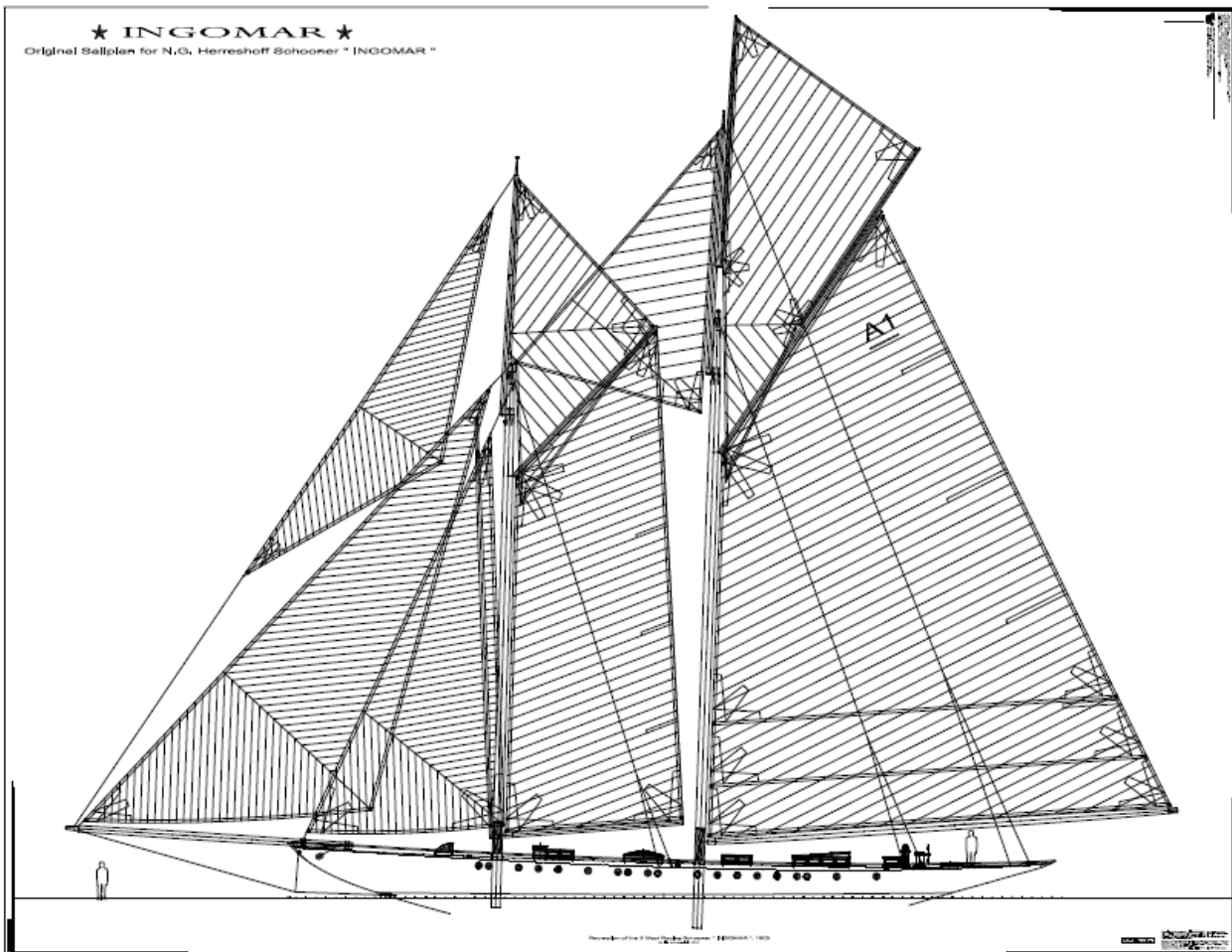
Figure 28 – Proposed Sailplan
